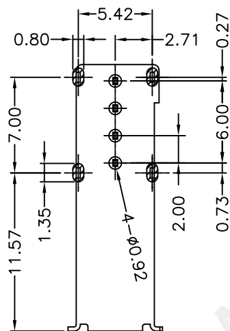
P.C.B LAYOUT TOP VIEW ±0.05
